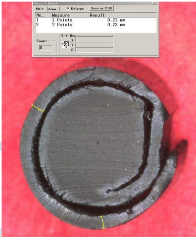
Fig. 9: O-ring damaged by gap extrusion (NBR 70 ShA at a gap of 0.2 mm and a pressure of 200 bar) in cross-section: atypically and strongly formed due to a sharp groove edge
